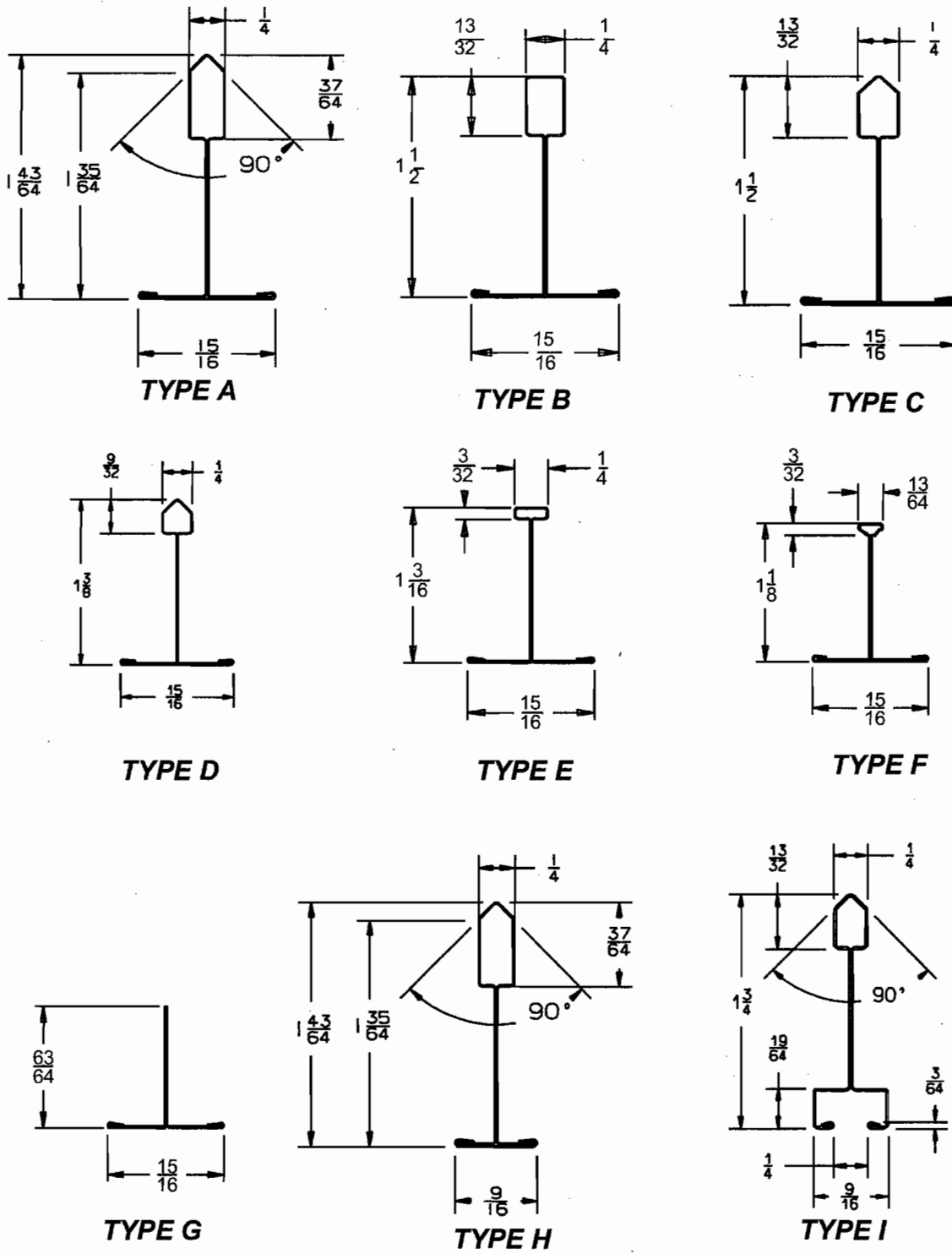
FIGURE 1—RUNNER PROFILES
